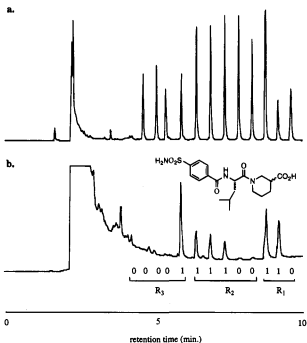
Figure 1. (a) Standard ECGC chromatogram showing the set of molecular tags used to encode library synthesis. (b) Representative encoding chromatogram from a bead identified in a carbonic anhydrase screen with the corresponding decoded structure.
