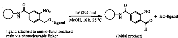
Scheme 2. Photolytic Cleavage of Ligand from Resin
