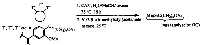
Scheme 3. Oxidative Release and Subsequent Decoding of Molecular Tags
